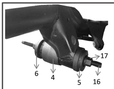
Installation-Front
