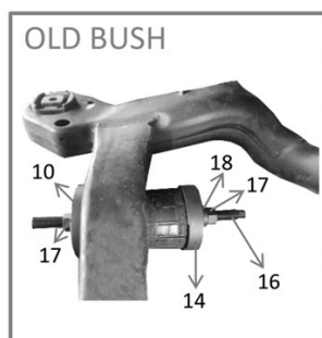
Installation- Rear
