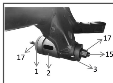
Removal-Front
