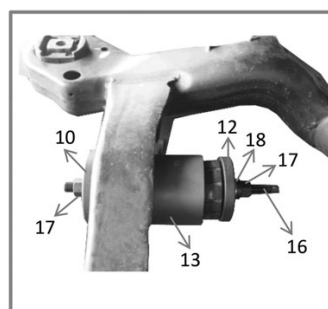
Installation- Rear
